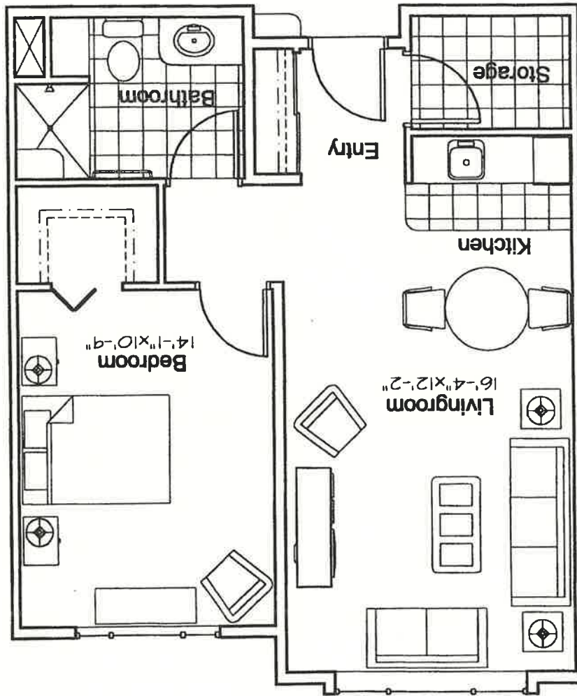
PLAN A - 1 BEDROOM 652 - 711 Sq. Ft.
